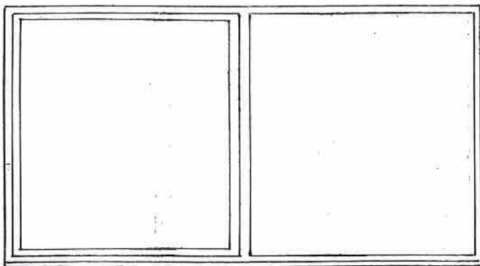
TYPE 2 - 1800 x 975mm.
